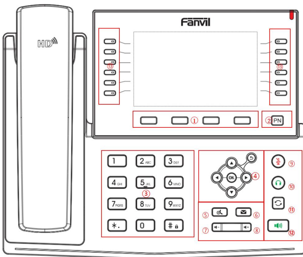
Picture 10 - Instruction of Keypad of X7C
