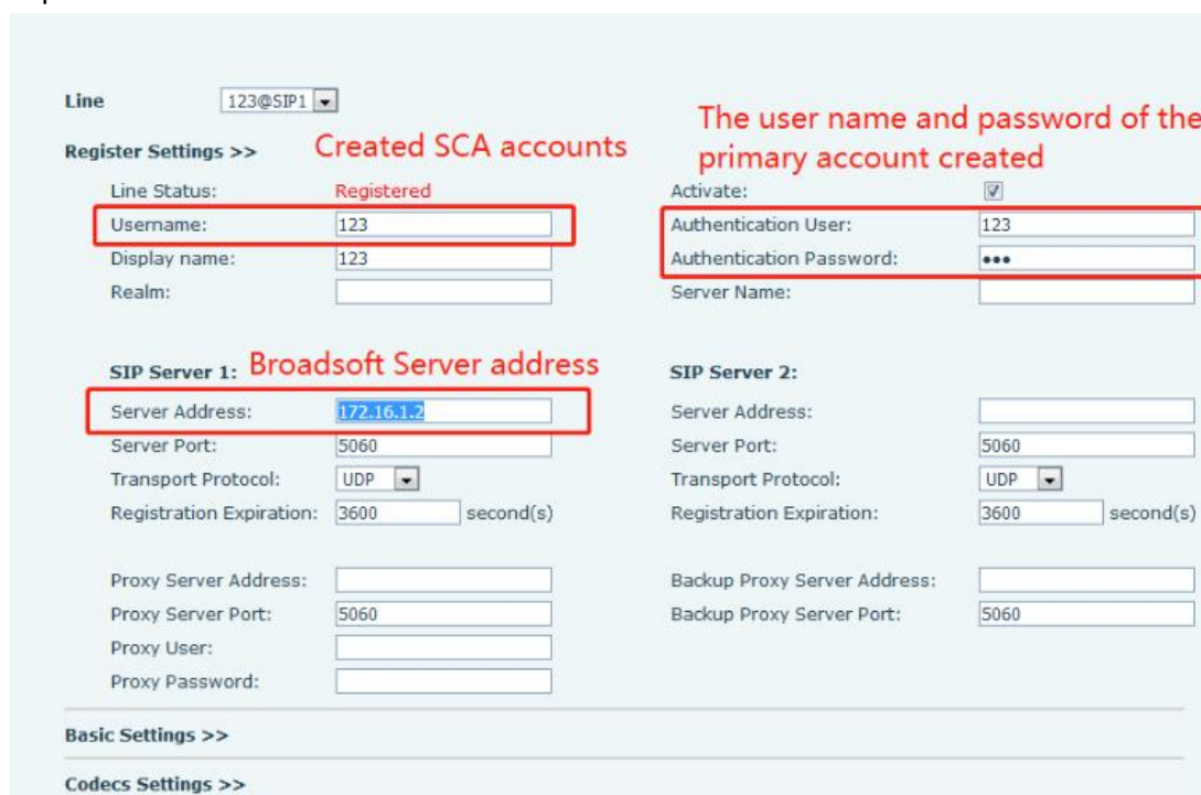
Picture 79 - Register BroadSoft account
